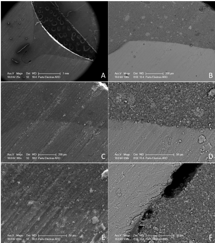
Figure 5. SEM micrograph of filled sealant sample with 100µm gap at different magnification
