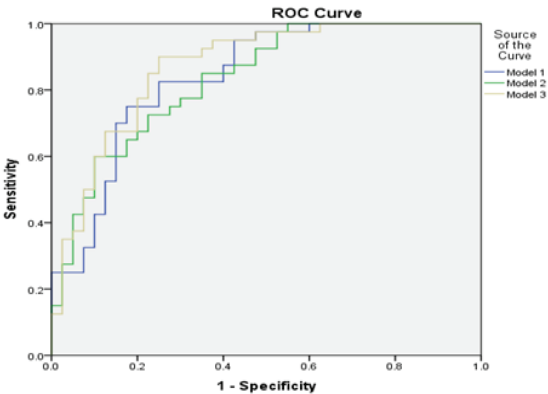
Figure 3. ROC curve
